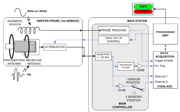
Fig. 2 - Simplified Sniffer hardware schematic.
