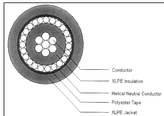
Figure 2: anti-robbery cable
